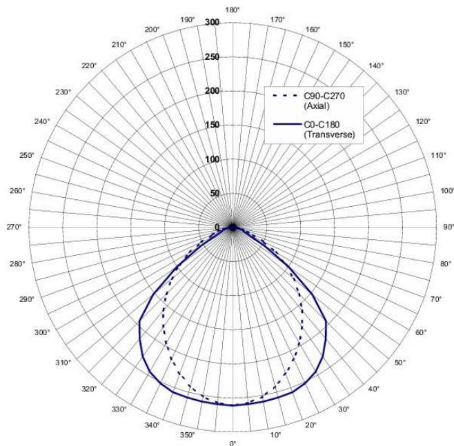
Approximate direct illumination at several distance from the luminaire centre
